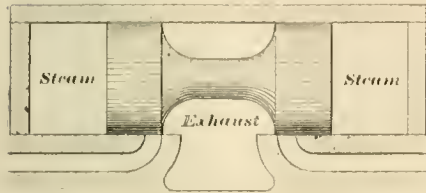
FIG. 2. PISTON VALVE—OUTSIDE ADMISSION.
